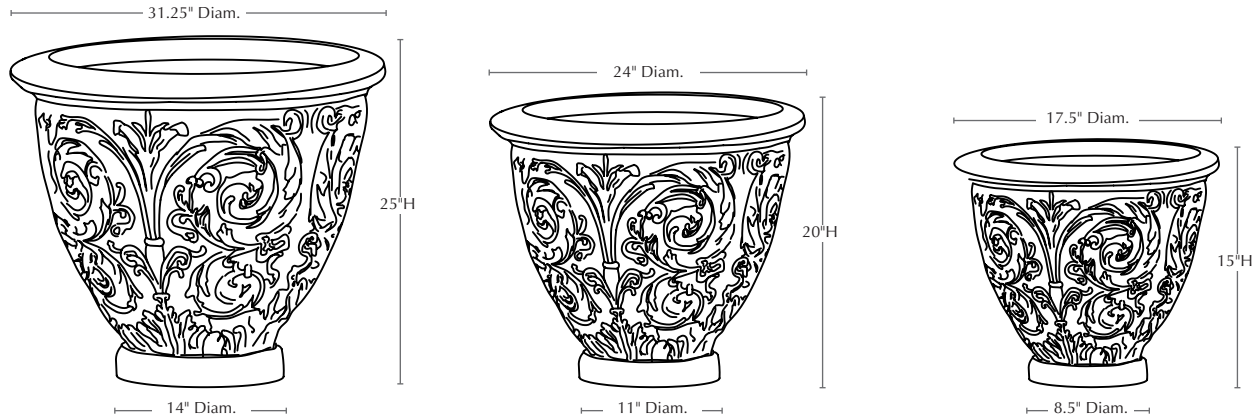
Isometric View
