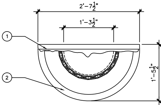
1 PLAN VIEW SCALE: 3/4"=1'
