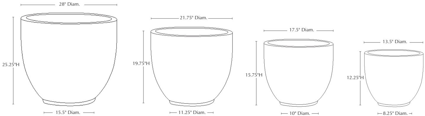
Isometric View
