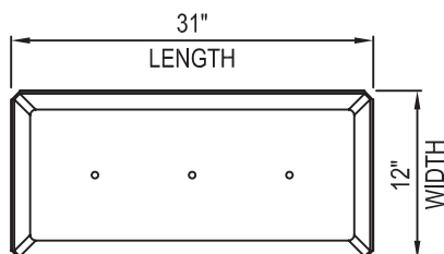
PLAN VIEWS
