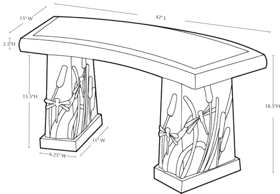
Isometric View
