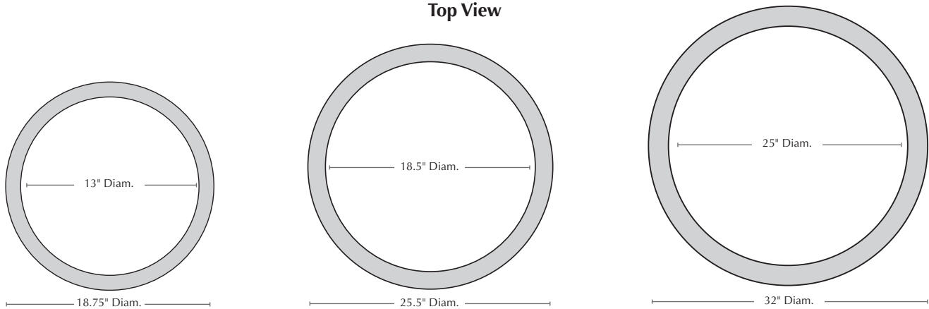
Top View
