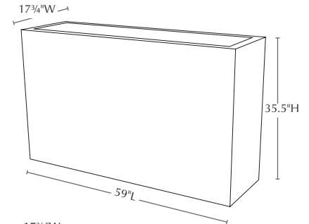
Isometric View
