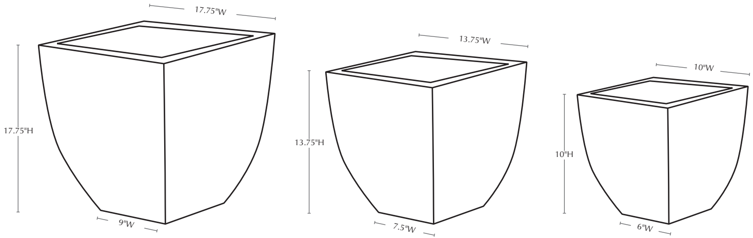
Isometric View
