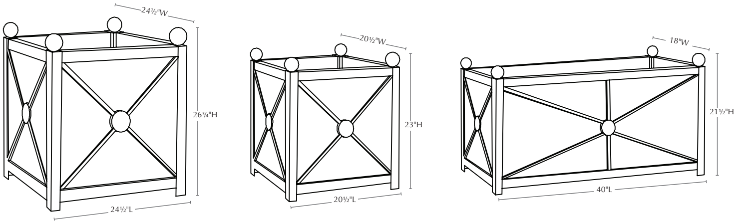
Isometric View
